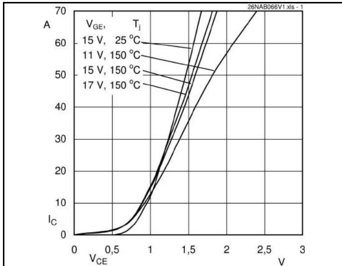
Fig. 1 Typ. output characteristics
