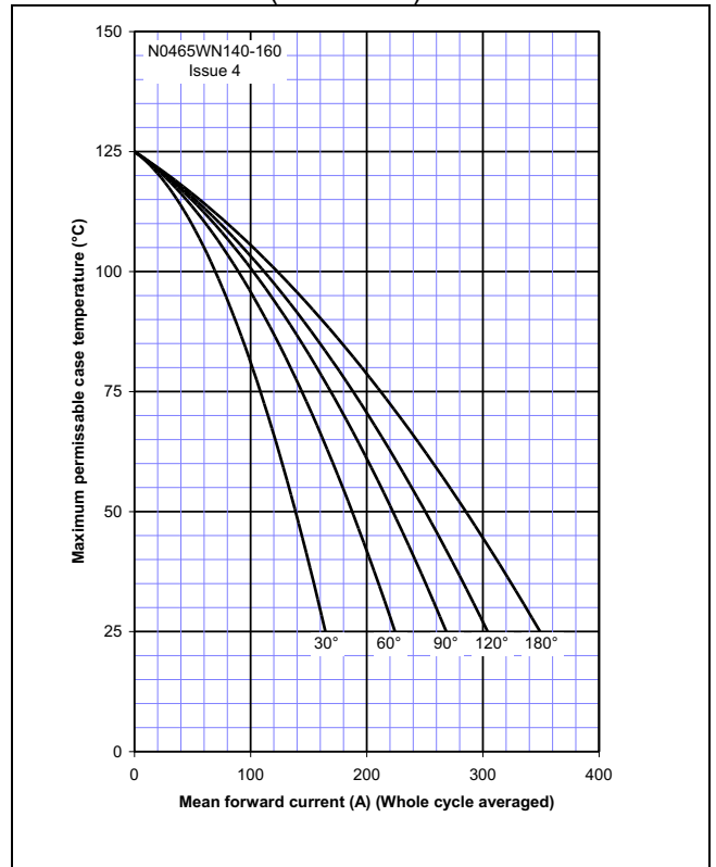
Figure 16 – On-state current vs. Case temperature – Anode Side Cooled (Square wave)
