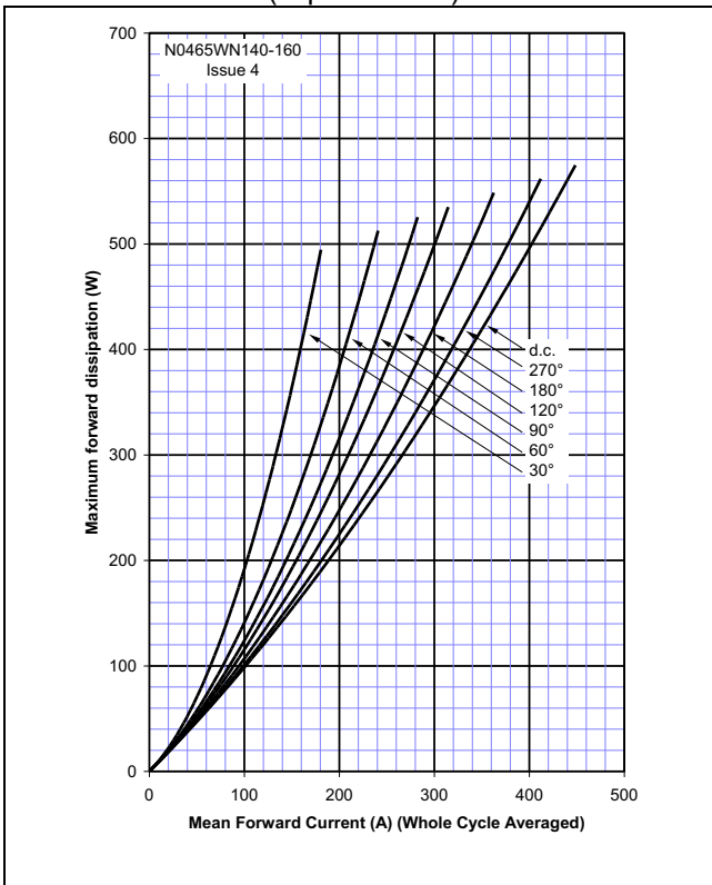
Figure 15 – On-state current vs. Power dissipation – Anode Side Cooled (Square wave)
